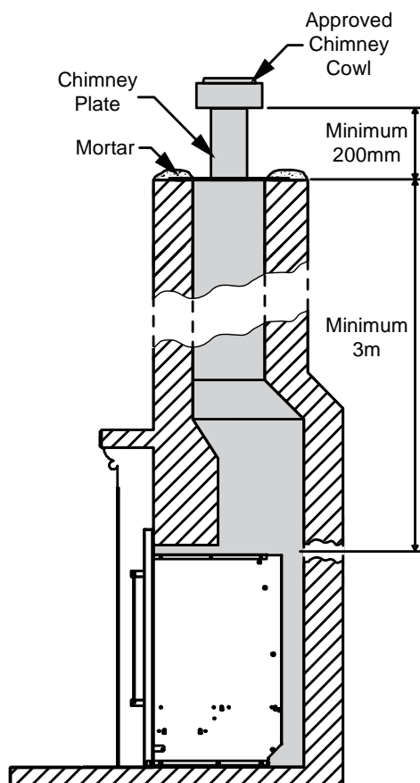
Open Chimney Installation
